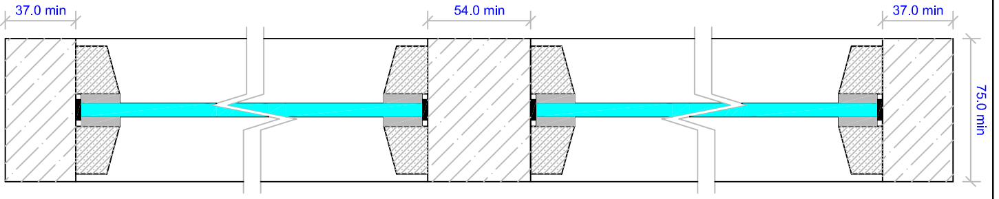
Vertical Through Sectional Drawing
